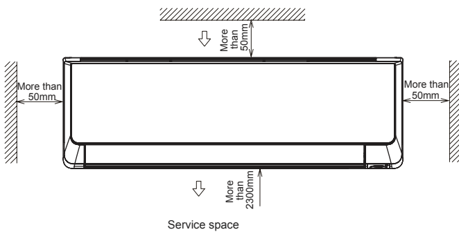
Service space
