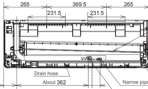
Wide pipe (φ 9.52) (RAK-25/35PXB)
