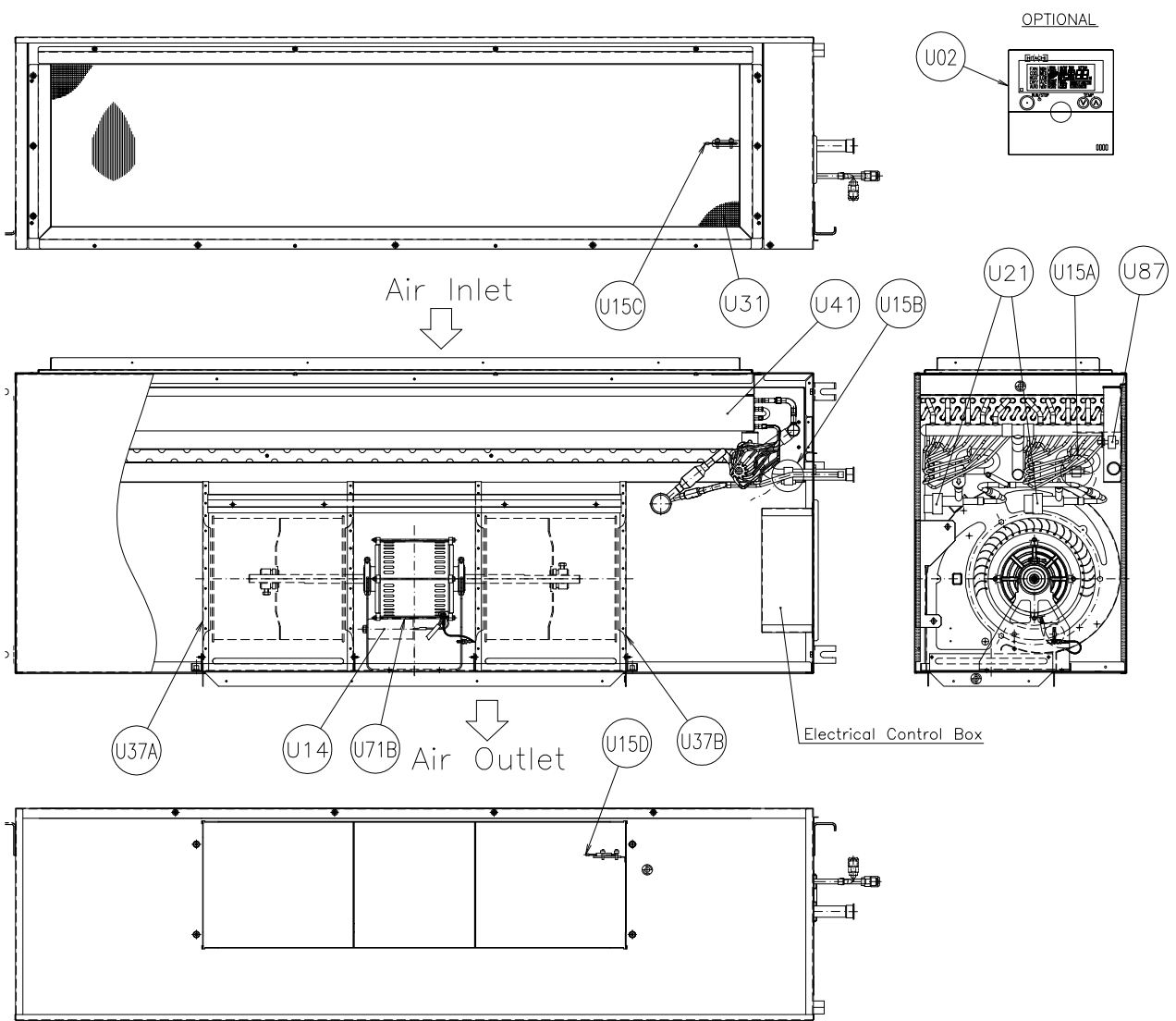
LOCATION OF ELECTRICAL EQUIPMENT IN THE ELECTRICAL BO
