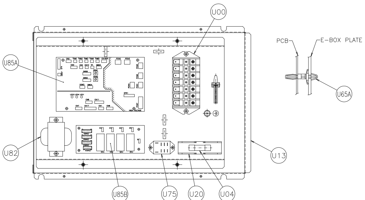
LOCATION OF ELECTRICAL EQUIPMENT IN THE ELECTRICAL BO
