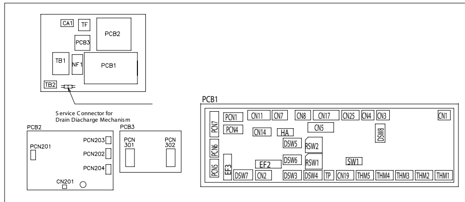
Printed Circuit Board
