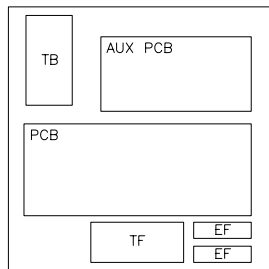
Electrical Box Lay-out
