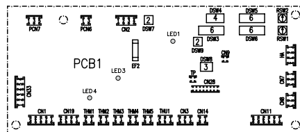
PCB1 Sockets Location
